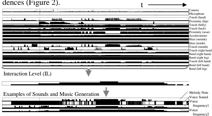
Figure 2: Sensor data, Interaction Levels, and Music Expression
