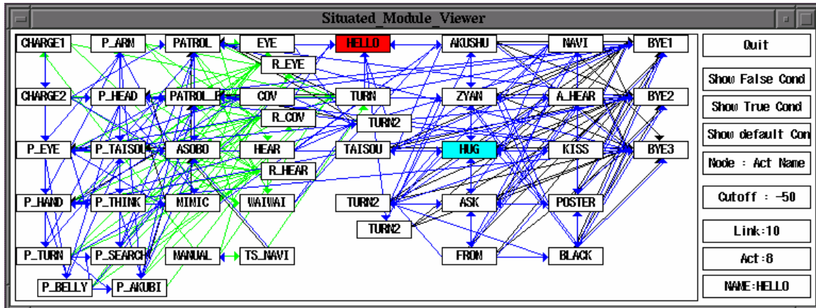
Figure 11: All behavior modules and their relationships
