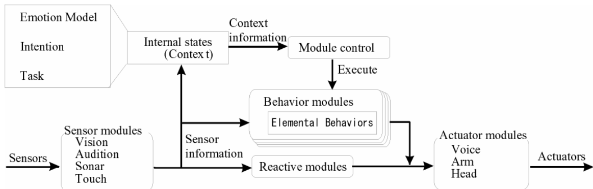
Figure 10: Software architecture based on behavior modules
