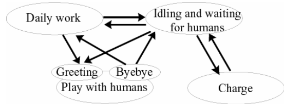
Figure 7: The meta-structure of the architecture
