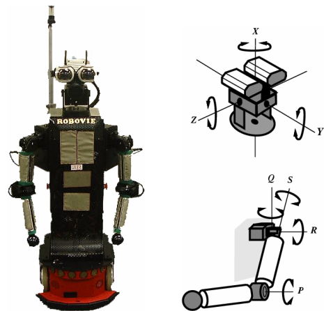
Figure 1: Robovie
