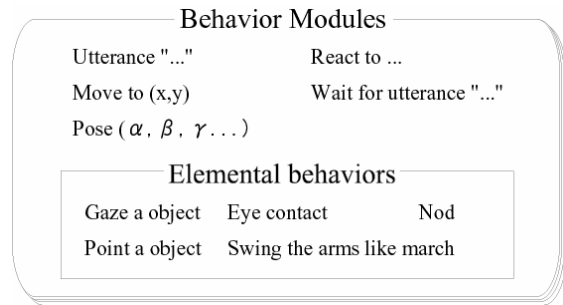
Figure 8: Behavior modules
